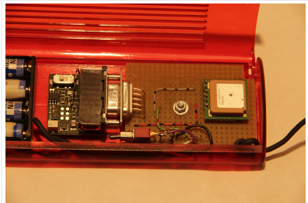
DXL APRS Tracker
