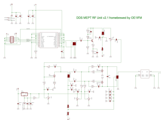
MEPT DDS & PA board circuit
