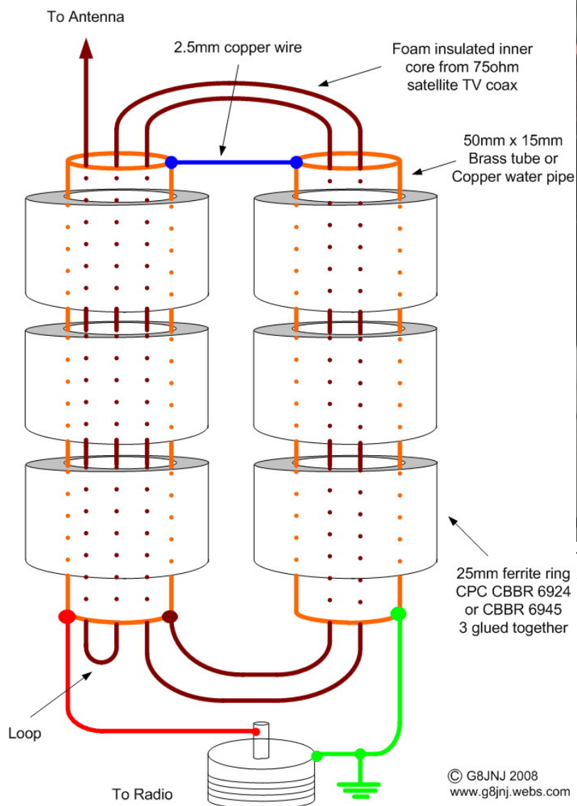
ransformator
