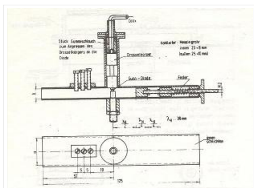
OE1RVW GUNN Mechanik
