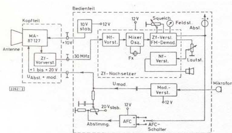
Abb. 2. 10-GHz-Transceiver, Blockschaltbild
