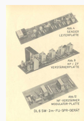
2m AM-Portabel, Transistorstation von DL9IW
