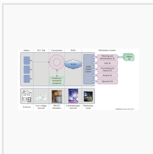
G3-PLC Network Architecture.jpg 1.329 × 679; 266 KB
